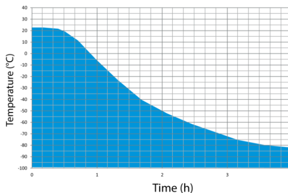
Pull-down time
